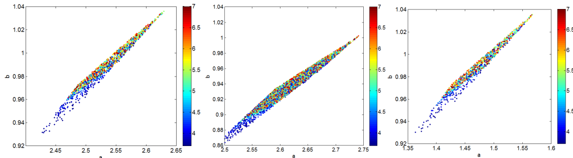
Figure 7: Scatterplots showing all realisations that comply with the data within a 1-sigma uncertainty. The color indicates the M_{max} of the realisation. The left figure shows the results of analysis 1 (BFMR, full period), the middle for analysis 2 (BFMR, 2003-2012), and the right for analysis 3 (normalized BGR, full period). The mean values are: analysis 1) a=2.53\pm0.04 , b=0.98\pm0.02 , and M_{max}=5.28\pm0.99 ; analysis 2) a=2.61\pm0.05 , b=0.93\pm0.03 , and M_{max}=5.29\pm0.98 ; analysis 3) a=1.47\pm0.04 , b=0.99\pm0.02 , and M_{max}=5.29\pm1.0 .
